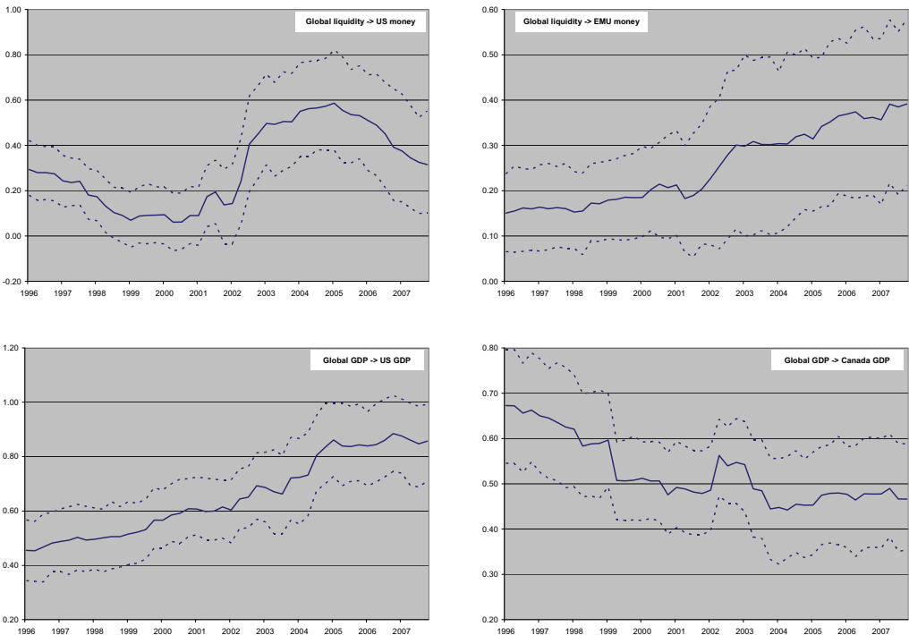
Chart 5 - Rolling regressions for factor loadings
