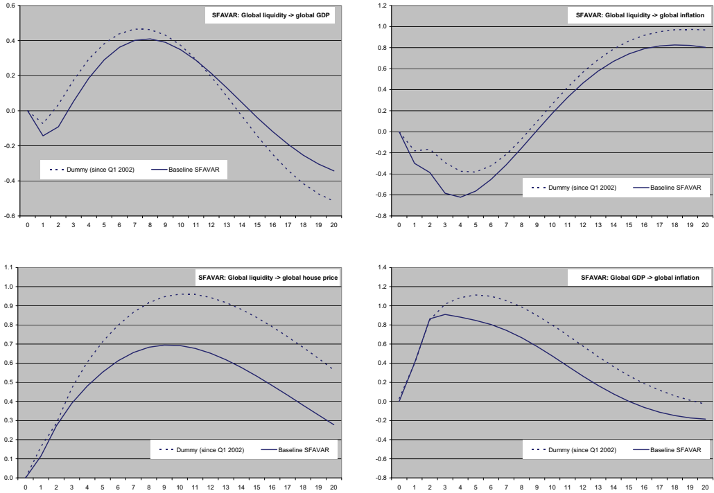
Chart 4 - Impulse response analysis in SFAVAR (dummy approach)
